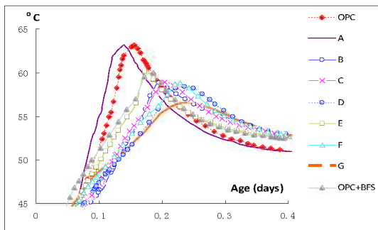
Fig 13 Internal temperature of mortars at 50°C
