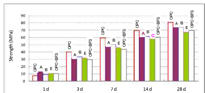
Fig 17 Compressive strength of some mortars
