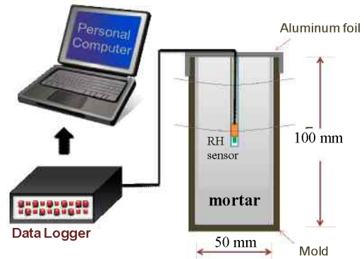
Fig 8 Internal relative humidity measurement
