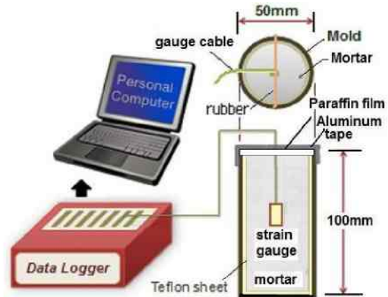
Fig 1 Autogenous shrinkage measurement apparatus
