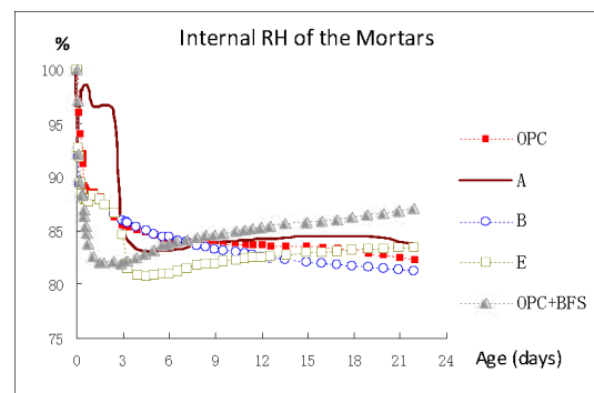
Fig 16 Relative humidity some specimens
