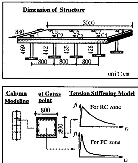
Figure 5 Structural Modeling
