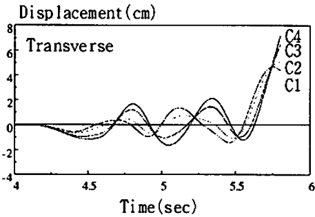
Figure 11 Response Displacement
