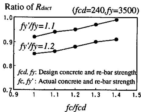
Figure 2 Variation of Shear to Moment Capacity with Material Strengths
