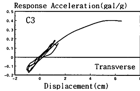
Figure 14 Hysteric Curve of Response Acceleration and Response Displacement in C3
