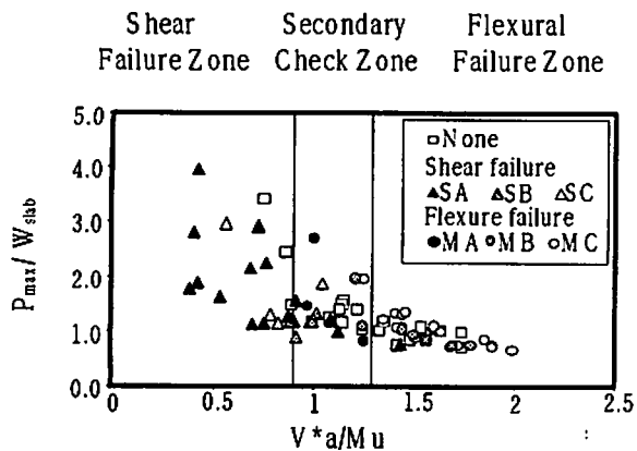
Figure 3 Failure Condition
