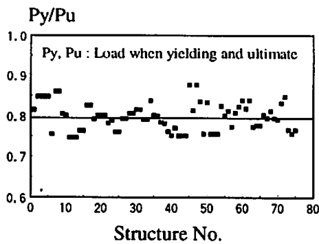
Figure 1 Ratio of Yielding to Ultimate Moment Capacity
