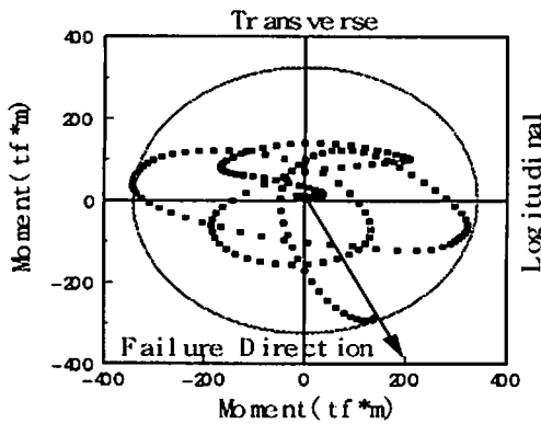
Figure 13 Interaction Diagram of Moment & Failure Envelop Curve
