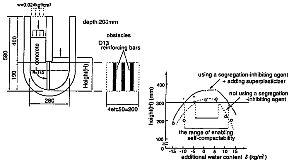
Fig.5 Improvement of self-compactability using a segregation-inhibiting agent
