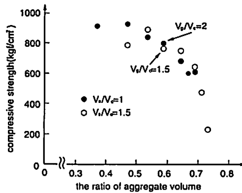
Fig.9 Variation of compressive strength with respect to the ratio of aggregate volume
