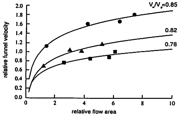
Fig.15 Relationship between relative flow area and relative funnel velocity
