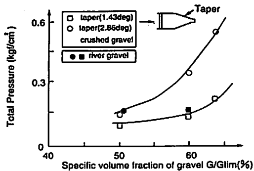
Fig.6 Total pressure at the inlet of tapered pipe with respect to the gravel content
