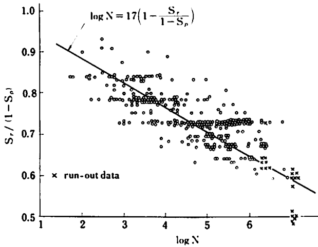
Fig.1 Fatigue strength of concrete in compression [4]-[8]
