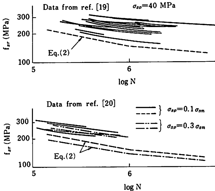
Fig.5 Fatigue strengths of reinforcing bars in tension
