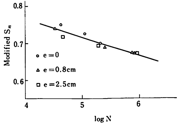
Fig.3 Ople and Hulsbos' data with modified ordinate by [11]
