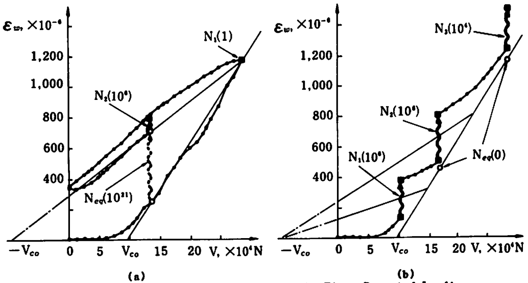
Fig.6 Average Strain of Stirrups after the First Repeated Loading
