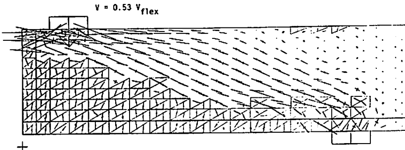
FIG.5 BEAM WITH CRACKING ALLOWED FOR ALL ELEMENTS
