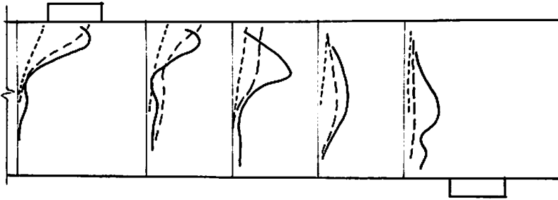
FIG.6 PREDICTED DISTRIBUTION OF COMPRESSIVE PRINCIPAL STRESSES FOR SHEAR 0.18, 0.44 AND 0.53 V_{flex}
