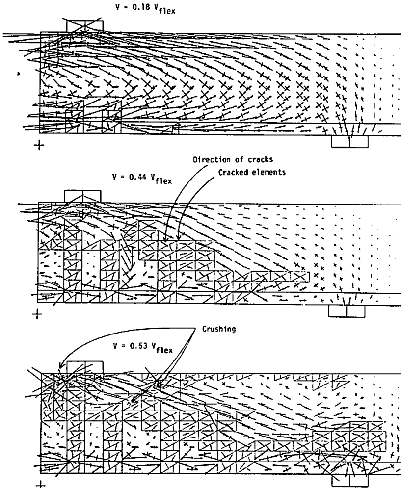
FIG.4 PREDICTED PRINCIPAL STRESSES, CRACKING AND CRUSHING
