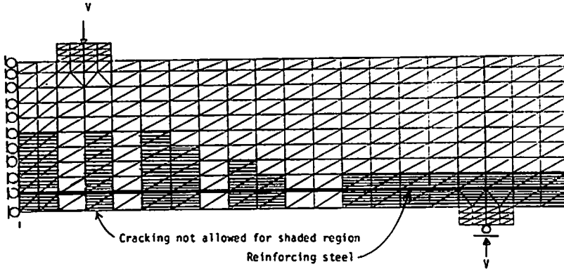
FIG.3 FINITE ELEMENT IDEALIZATION
