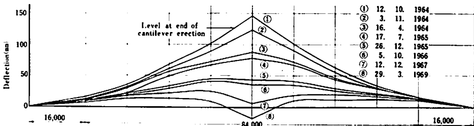
Fig. 3. Change of deflection at Yagiyama highway bridge
