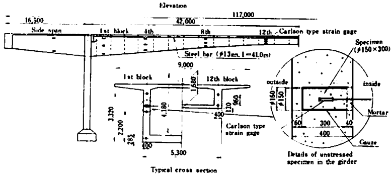
Fig. 1. Gage arrangement of Yagiyama highway bridge
