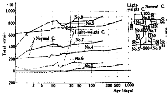
Fig. 8. Measured deformations in light-weight aggregate and normal gravel concrete girders with same section
