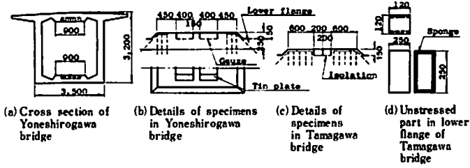
Fig. 4. Arrangement of concrete specimens for cut-out
