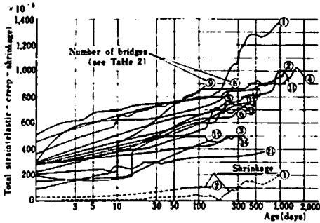
Fig. 6. Summary of measurements of delayed deformations in prestressed concrete bridges
